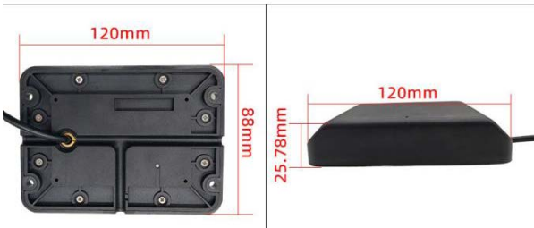
Sensor size: 120*88*25.78mm
